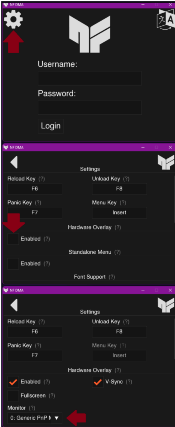
Nightfall No-Fuser
